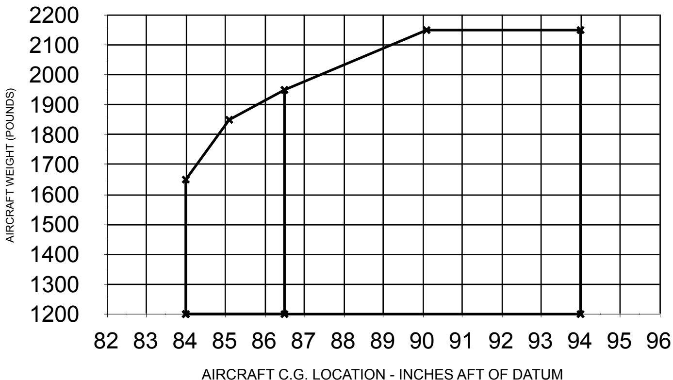
Center of Gravity Graph - PA-28-140 (N6469W)
